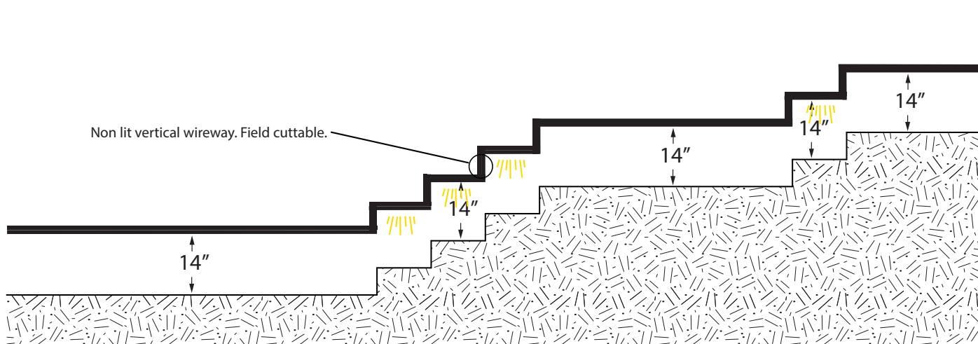
90° Vertical Outside
